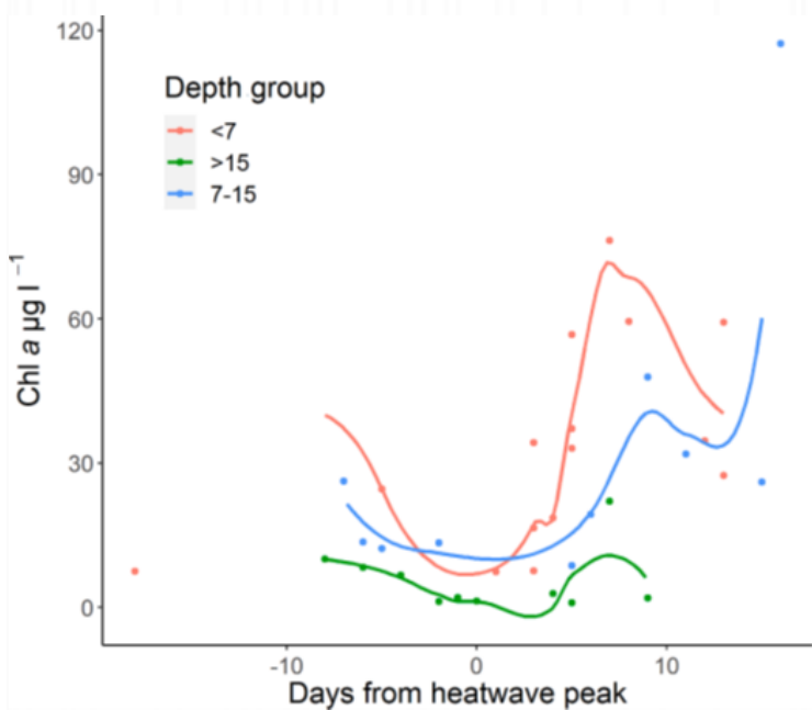
Figure 3. Timing and concentration of peak chlorophyll-a with respect to the second 2019 heatwave. Lakes coloured and lowess smoother (a locally weighted non-parametric smoothing method) applied by mean depth group. Source: Free et al. 2022.
