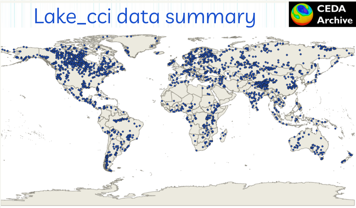
Figure 1. The first Climate Research Data Package (CRDP V2.0.2, 2022) was recently created.
