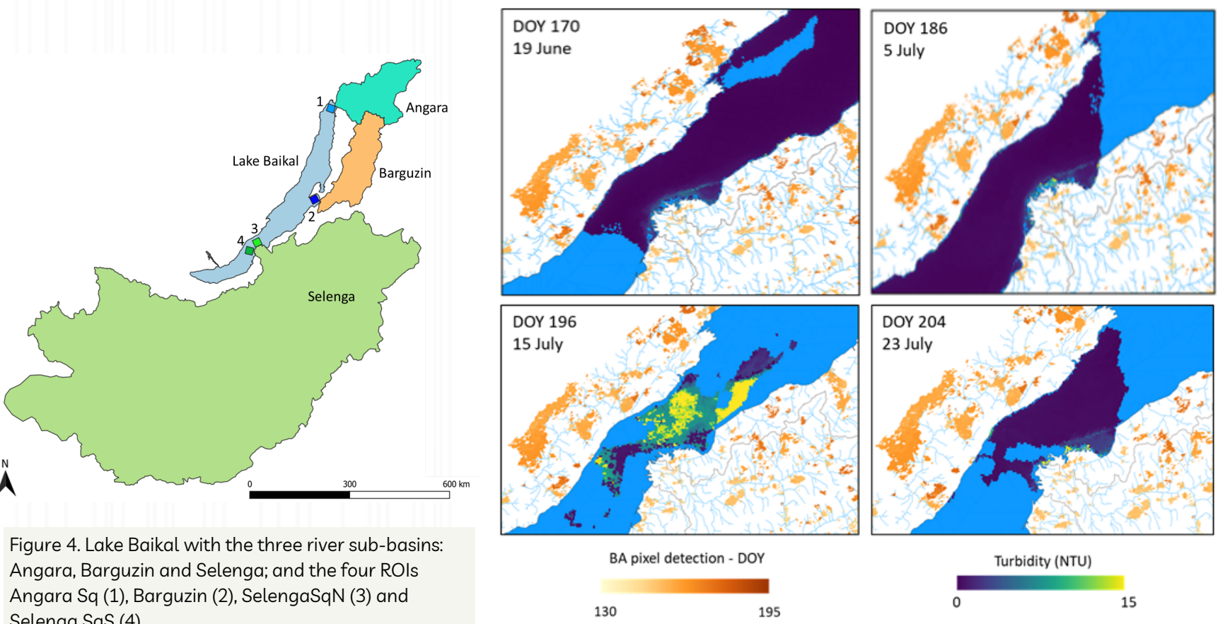
Figure 6. Maps of turbidity (NTU) and burned area (BA) in relation to the day of year (DOY) in 2003 for the central portion of Lake Baikal.
