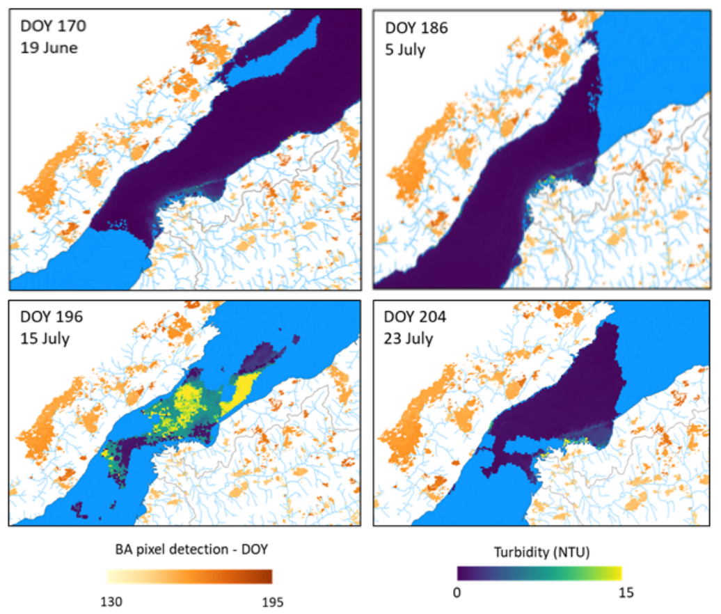
Figure 6. Maps of turbidity (NTU) and burned area (BA) in relation to the day of year (DOY) in 2003 for the central portion of Lake Baikal.
