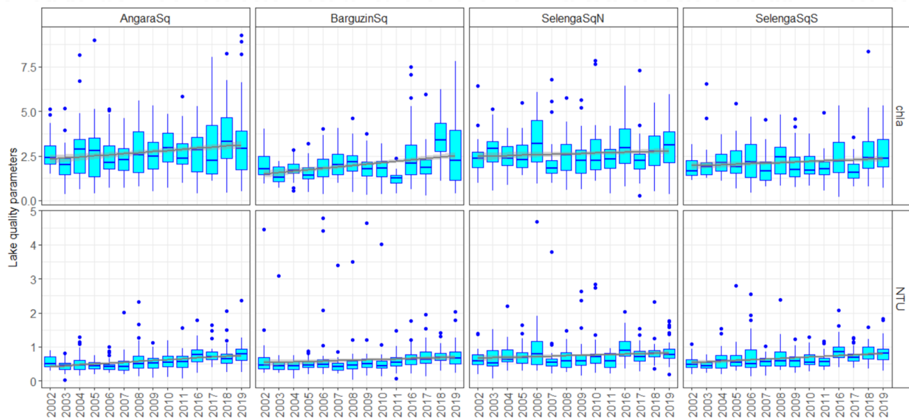
Figure 5. Trends of chlorophyll-a (chl-a), turbidity (NTU) in the four ROIs (Region of Interests; Angara Sq, Barguzin, SelengaSqN and Selenga SqS) close to the inflow of the main tributaries into the Lake Baikal.
